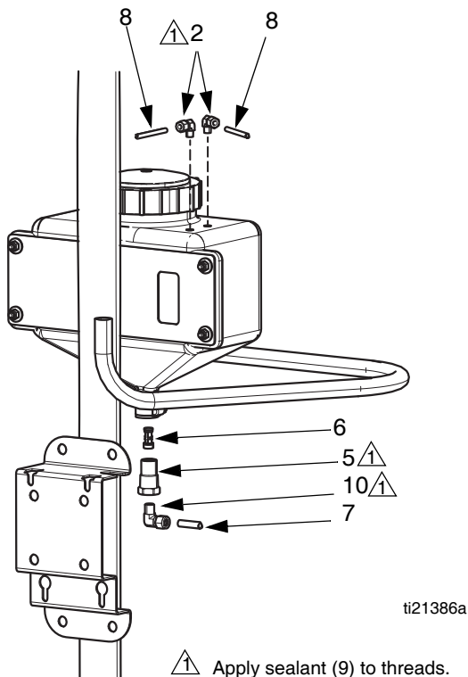
FIG. 1: Catalyst Reservoir
