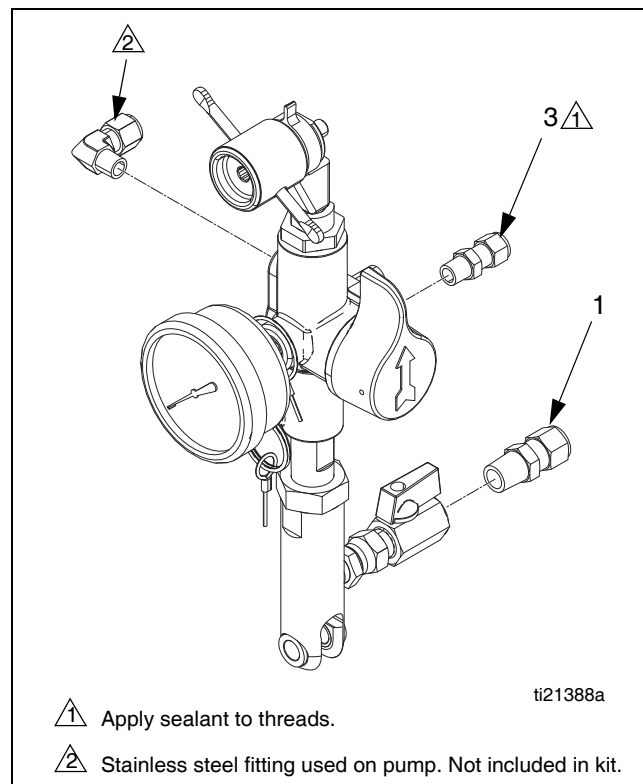
FIG. 2: Catalyst Pumps
